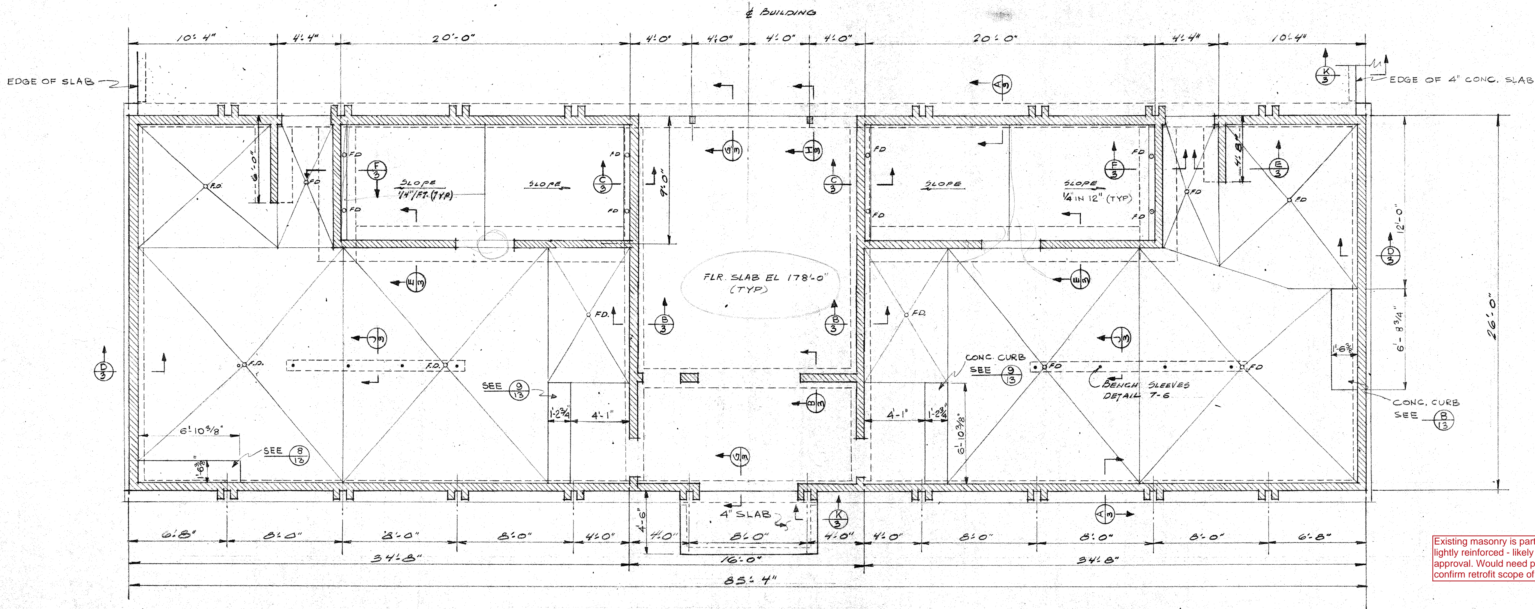
FOUNDATION PLAN - BATH HOUSE SCALE: 1/4" = 1'-0"
