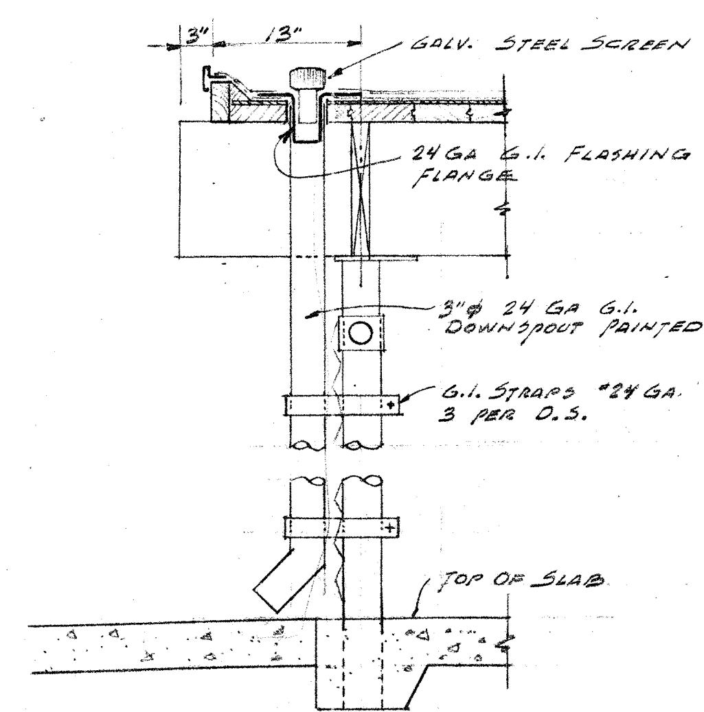
DOWNSPOUT DETAIL SCALE: 1" = 1'-0"
