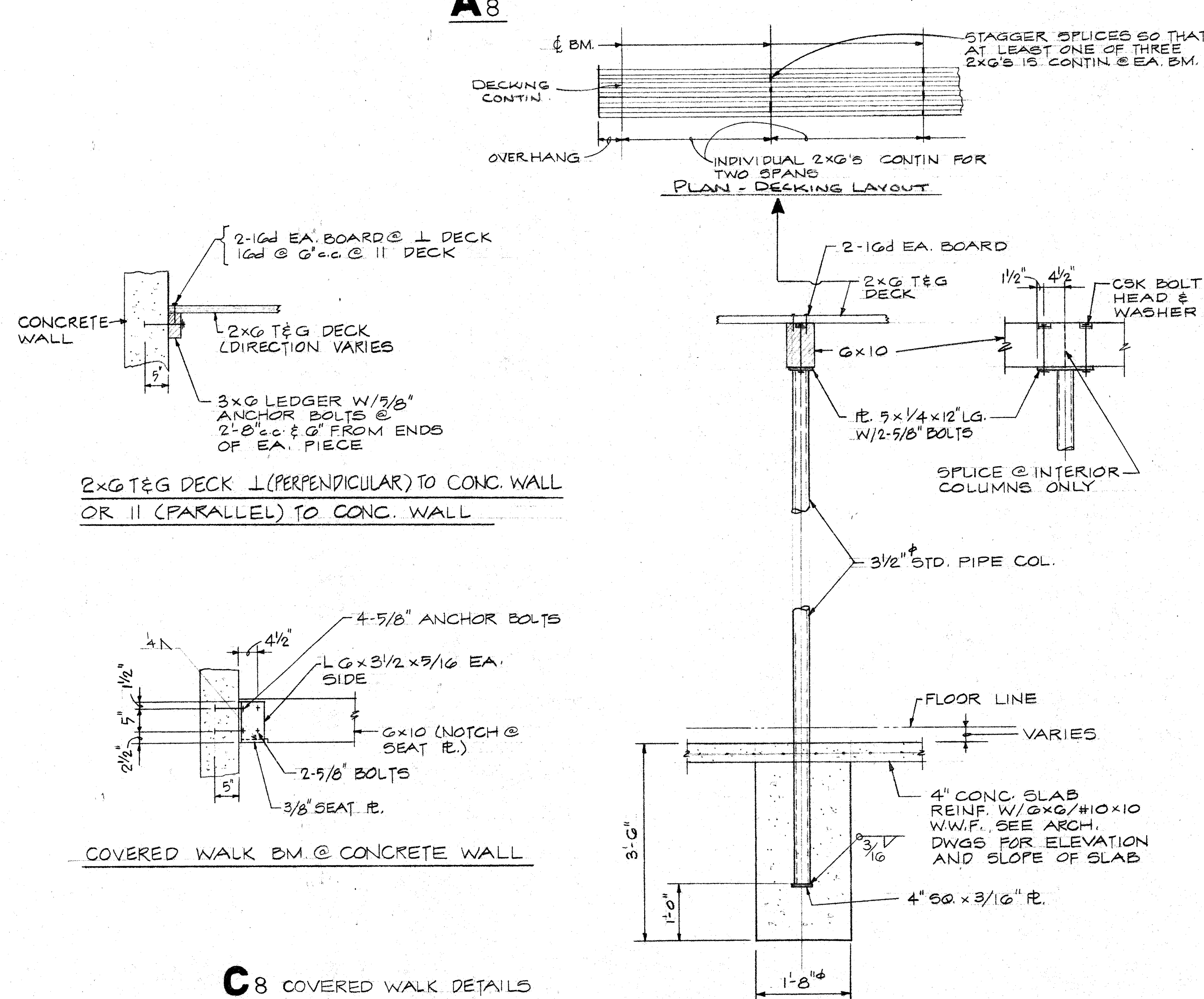
TYPICAL COVERED WALK COLUMN
