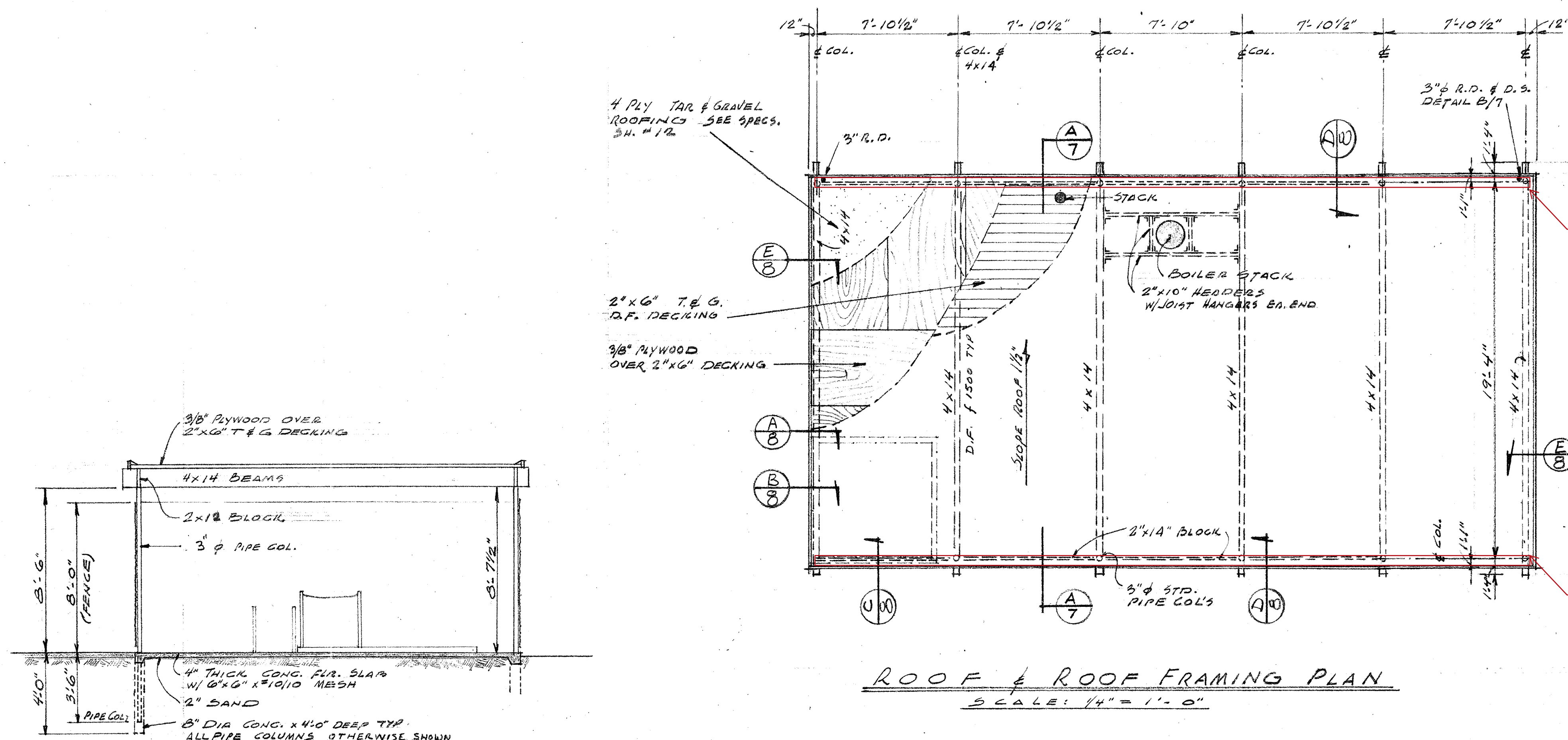
TYP. CROSS SECTION SCALE: 1/4" = 1'-0"
